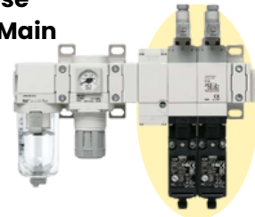
Direct Operated/Pilot Operated 2-Port Solenoid Valve JSX/JSX
