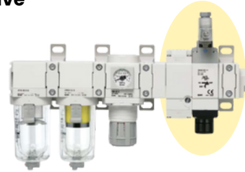
3-Port Solenoid Valve/ Residual Pressure Release Valve with Detection of Main Valve Position VP546/746
