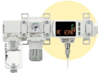
3-Color Display Digital Flow Switch PF3A7/8[ ]H(-L)
