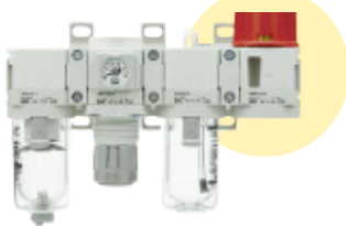
OSHA Standard Compliant Pressure Relief 3- Port Valve with Locking Holes (VHS[ ]-D/VHS[ ]W-D)
